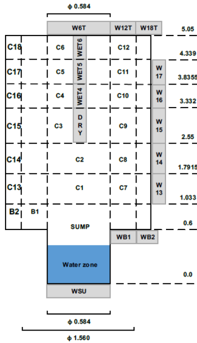
Figure 1: MELCOR nodalization.
